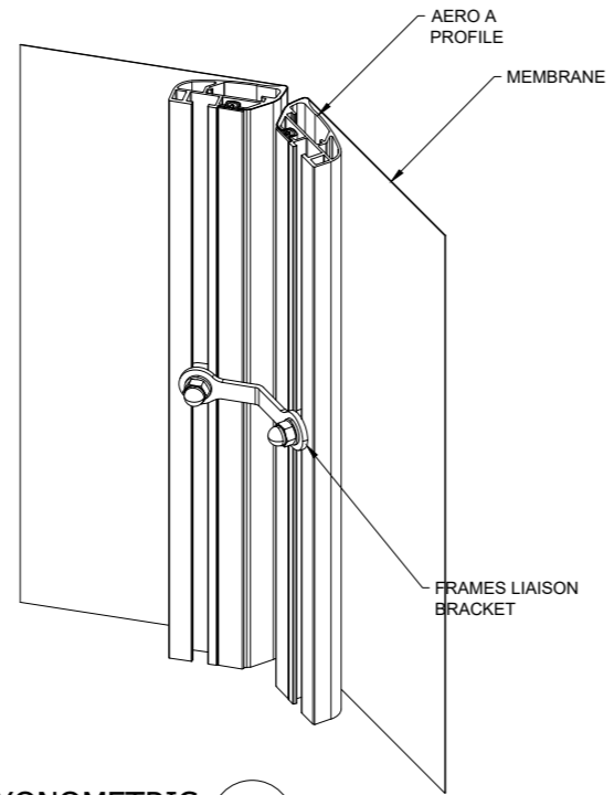
AXONOMETRIC VIEW 1:5
