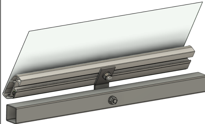
AXONOMETRIC VIEW 1:2
