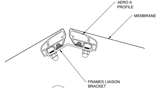
SECTION DETAIL 1:5
